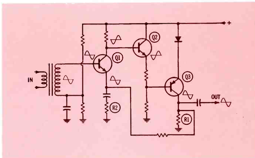
Fig. 2. Feedback voltage is applied to first-stage emitter in this circuit.
