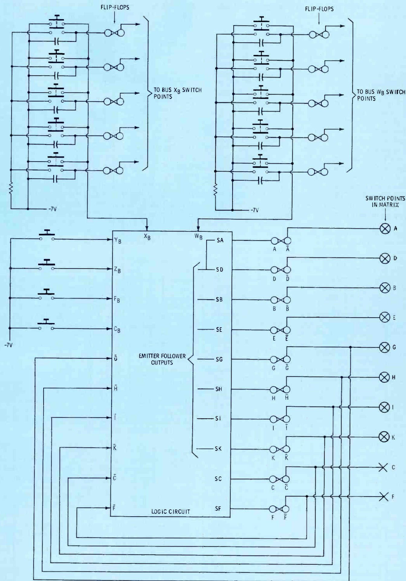
Fig. 3. Logic-circuit control diagram shows how flip-flops are connected to the switching matrix through logic card.
