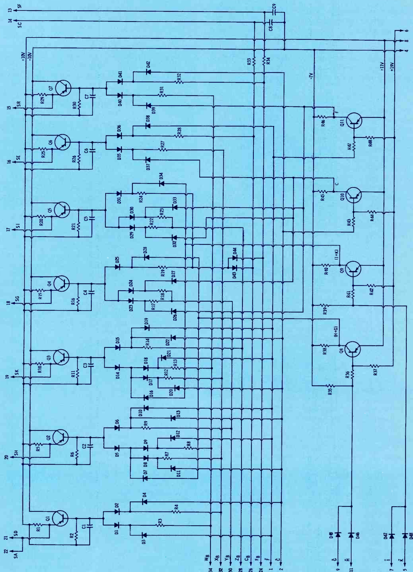
Fig. 2. Logic-card circuit indicates diode gates, emitter followers Q1 through Q7, and inverters Q8 through Q11.
