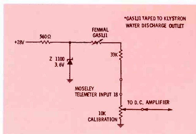
Fig. 14. Temperature problems detected with this circuit.
