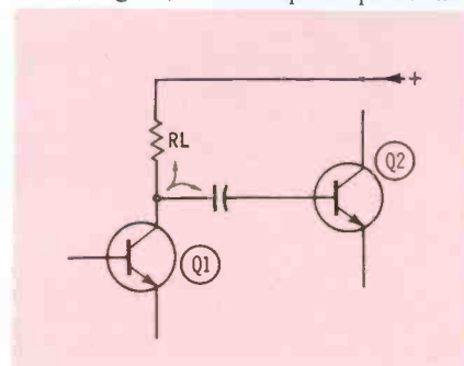
Fig. 7. High value of load R cannot be used to divert Q1 output signal.
