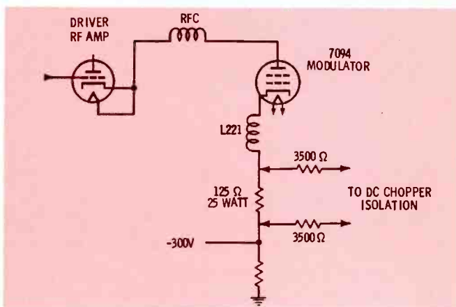
Fig. 13. Driver-modulator sensing circuit uses chopper.
