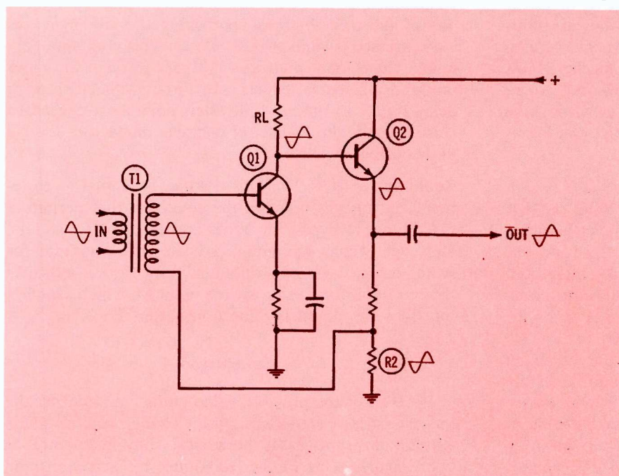
Fig. 1. Two-stage microphone preamplifier obtains negative feedback from R2.
