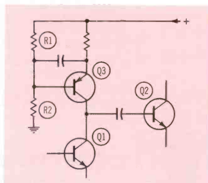
Fig. 8. Electronic choke replaces R_{L1} .
