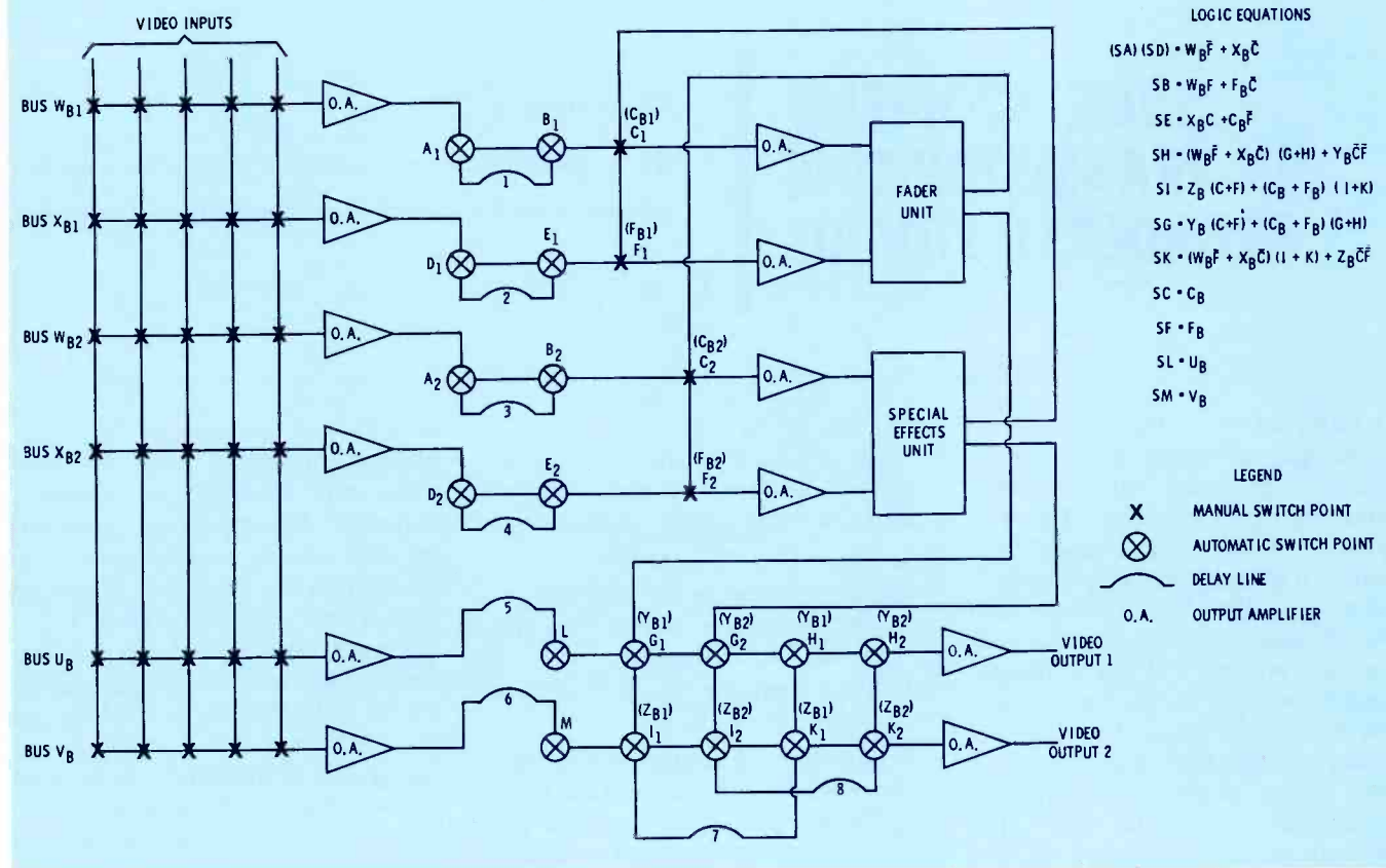
Fig. 4. Typical switching matrix for system including fader and special-effects units with useful logic equations.
