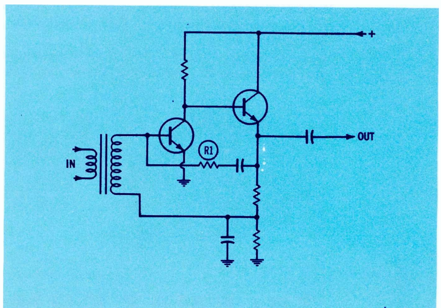
Fig. 11. Negative feedback reduces the input impedance of mixing amplifier.
