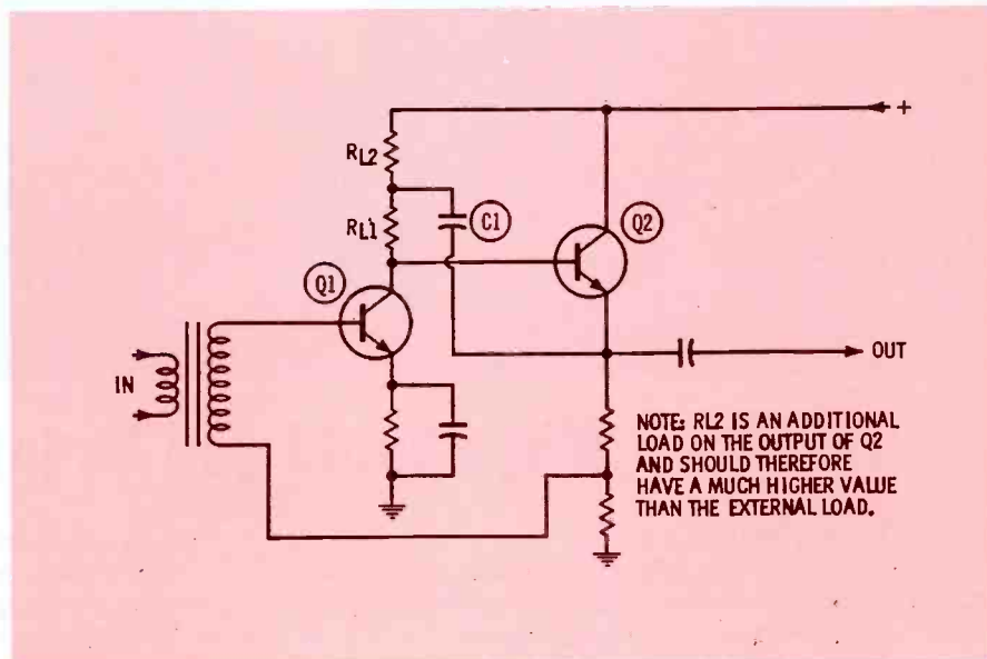
Fig. 3. "Bootstrapping" arrangement prevents partial loss of signal current.
