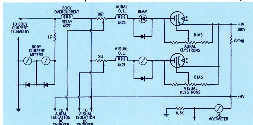
Fig. 12. One-ohm resistor senses klystron and body current in this circuit.
