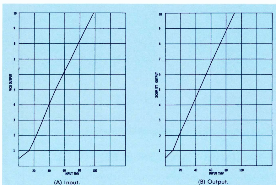
Fig. 10. Curves show PBR linearity after the modifications had been completed
