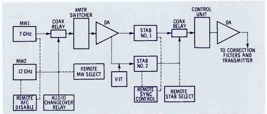
Fig. 1. Video flow as it evolved for the KCET remote-control installation.
