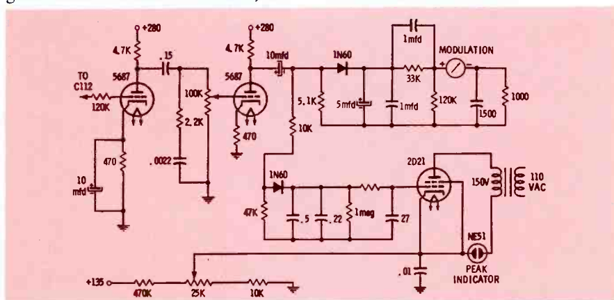
Fig. 15. Additions to studio monitor are used to monitor audio modulation.
