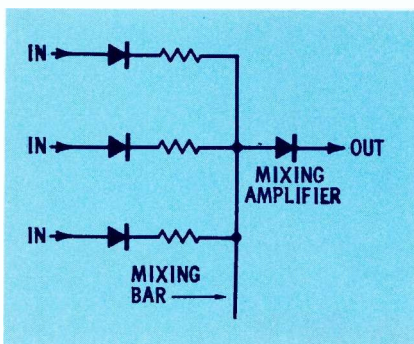
Fig. 10. Typical audio mixing method.
