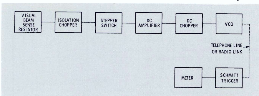
Fig. 8. Typical metering circuit which employs DC chopper and DC amplifier.
