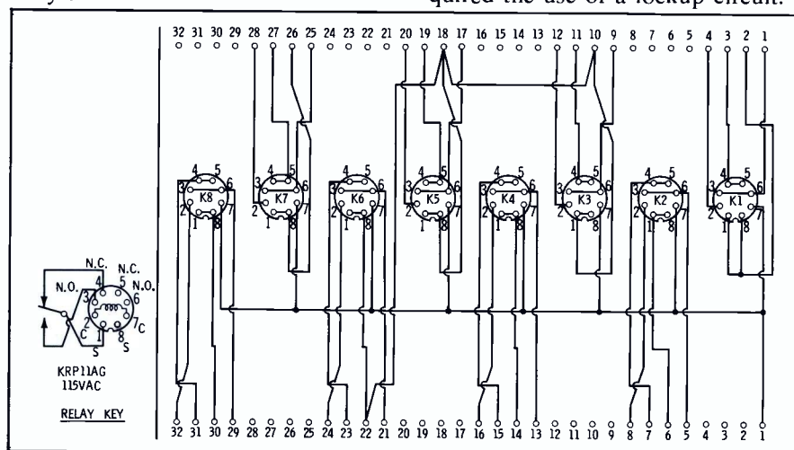
Fig. 16. Wiring diagram for typical basic unit of relay logic control unit.
