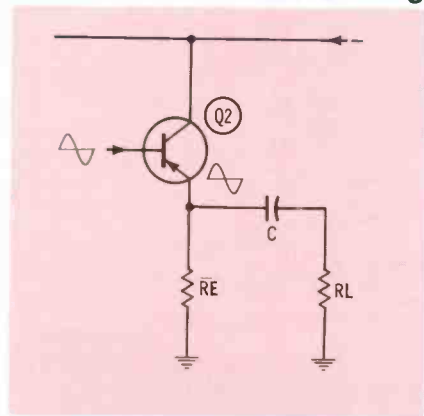
Fig. 4. Part of output signal current is diverted through emitter resistor.
