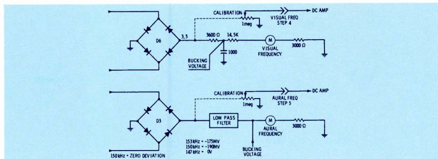
Fig. 11. Sensing circuits employed to measure aural and visual frequencies.
