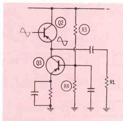
Fig. 5. Second transistor acts as an emitter-circuit "electronic choke."
