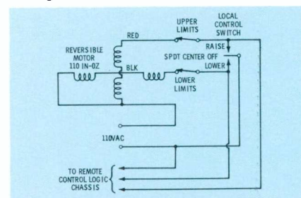
Fig. 6. Miniature switches limit motor rotation to 300° for power control.
