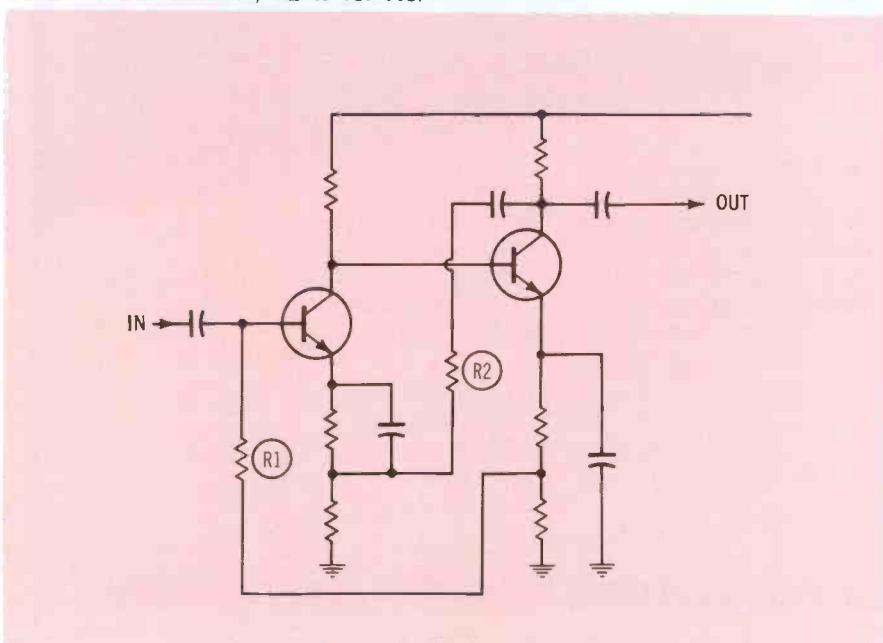
Fig. 6. Intermediate-level amplifier; R1 is for DC feedback, R2 is for AC.
