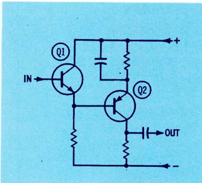
Fig. 9. Use of complementary transistors improves temperature stability.
