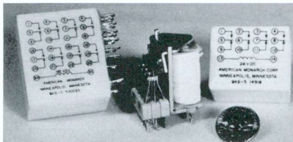
Telephone-Type Relay (54)
