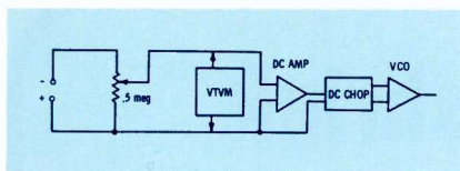
Fig. 9. Test setup for calibrating remote-control linearity after changes.
